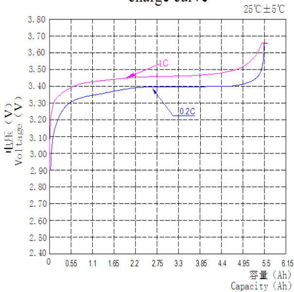
充电曲线图 charge curve
